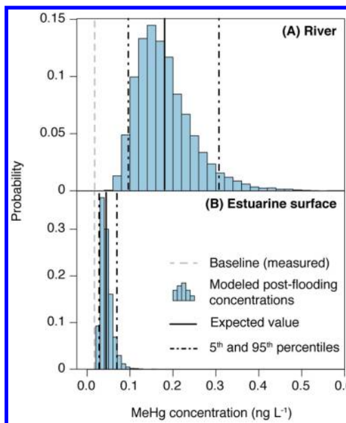
Figure 3. Probabilistically modeled scenarios for MeHg increases in downstream river and estuary of the Muskrat Falls hydroelectric facility. Photochemical MeHg demethylation is assumed to occur continuously down the reach of the Churchill River into Lake Melville thus the river concentration reflects the average of reservoir concentrations and downstream inputs to Lake Melville.
